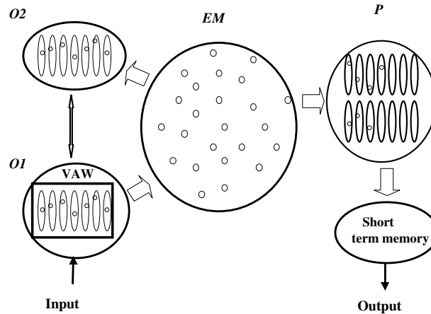
Fig. 1. Architecture of the multitrace connectionist model of reading (Ans et al., 1998); O1 = input orthographic layer, O2 = orthographic echo layer, EM = episodic memory, P = output phonological layer, VAW = visual attentional window. The phonological and orthographic layers are sets of unconnected clusters of elementary units coding for phonemes and alphabetic characters respectively. The arrows depict fully distributed modifiable connections. The double arrow symbolises a matching check procedure comparing the identity of the orthographic echo generated over O2 with the O1 input pattern. Units within the VAW are maximally and equally activated.
